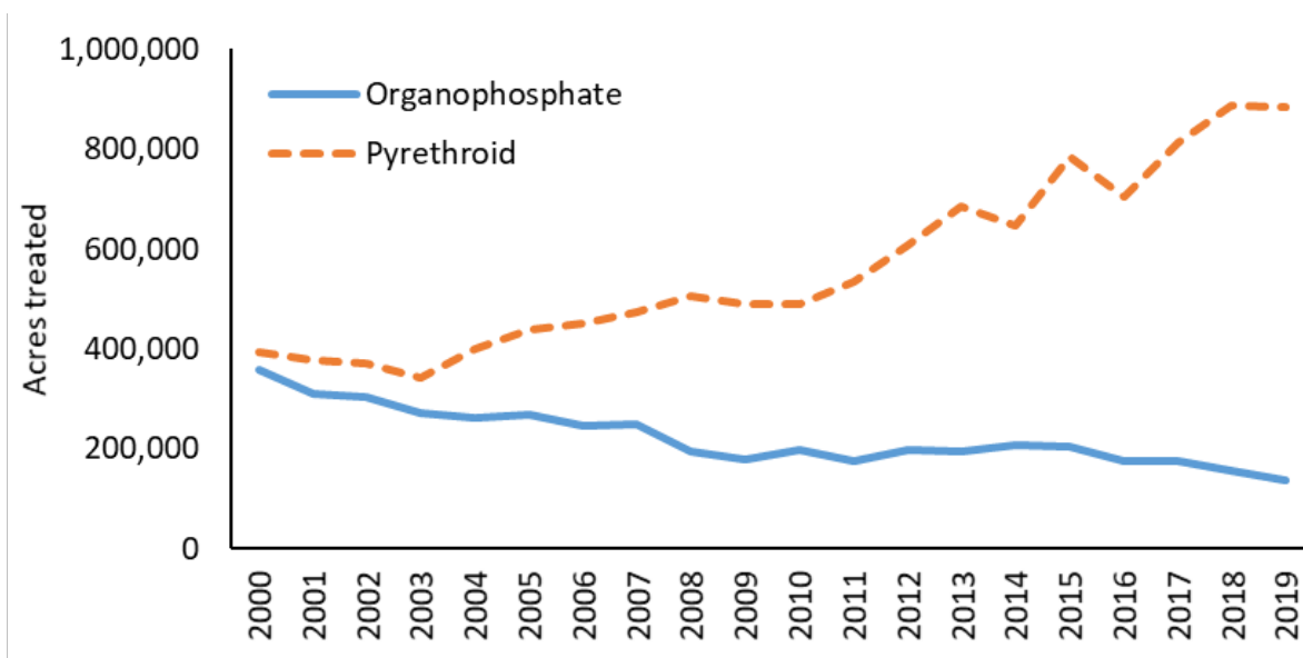
Figure 1. Annual acres treated with organophosphate and pyrethroid insecticides in the Sacramento Valley from 2000 to 2019. Source: California Department of Pesticide Regulation Pesticide Use Report data.
