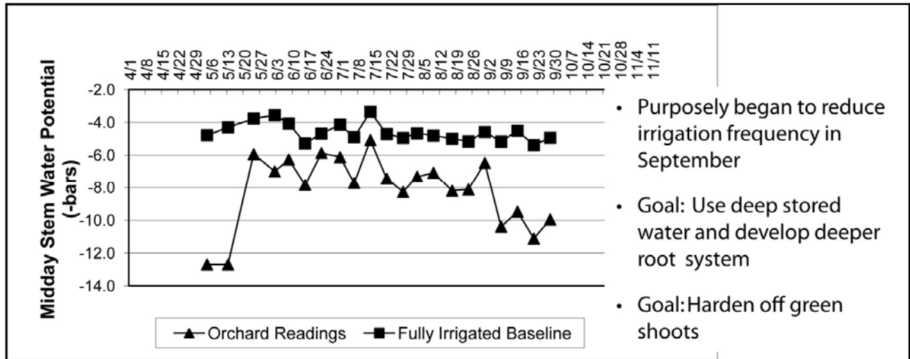
Figure 2. Example of how a pressure chamber SWP is used to manage irrigation in a first leaf walnut orchard. The baseline represents SWP when soil moisture is not limiting ET.
